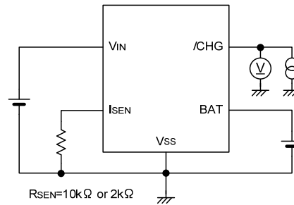
6. Soft-start
