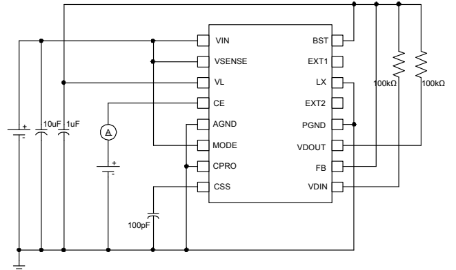
Circuit 19
