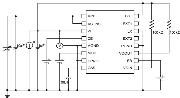
Circuit 23
