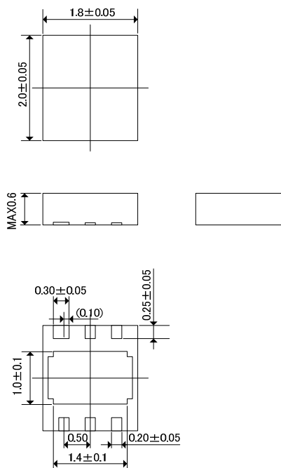
USP-6C Package
