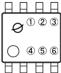
SOP-8 (TOP VIEW)
