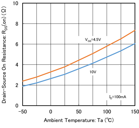
(4) Drain-Source On-State Resistance vs. Ambient Temperature
