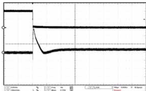
XC9220x095xx ( 500kHz, PWM制御 ) VIN=10.0V, VOUT=3.3V VOUT : 100mV/div, Time : 100usec/div
