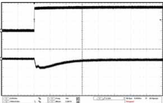
XC9220x095xx ( 500kHz, PWM制御 ) VIN=10.0V, VOUT=3.3V VOUT : 100mV/div, Time : 50usec/div
