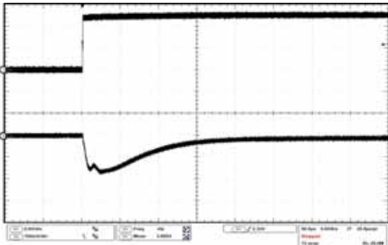
XC9220x095xx ( 500kHz, PWM制御 ) VIN=5.0V, VOUT=3.3V VOUT : 100mV/div, Time : 50usec/div
