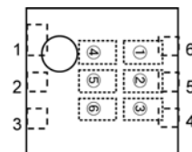
USP-6C (TOP VIEW)
