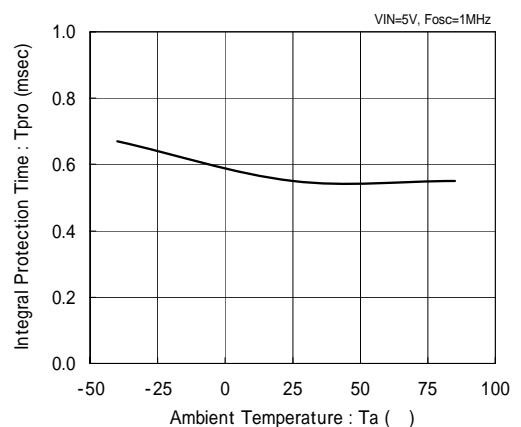
XC9220/21A, Bseries
