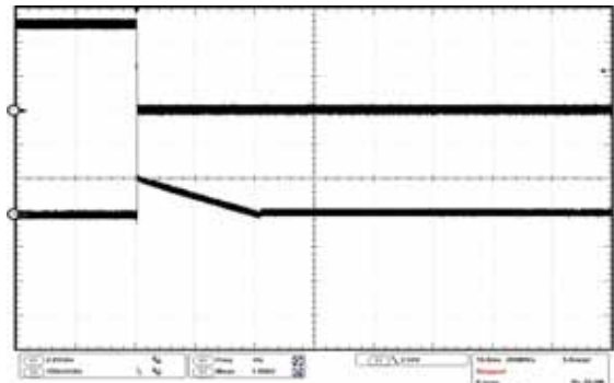
XC9220x095xx ( 500kHz, PWM制御 ) VIN=5.0V, VOUT=3.3V VOUT : 100mV/div, Time : 10msec/div
