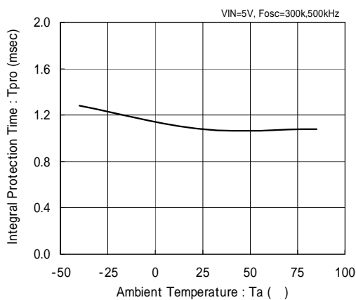
XC9220/21A, Bseries
