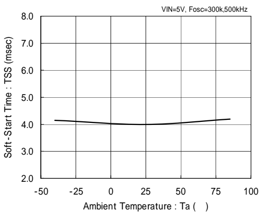
XC9220/21series
