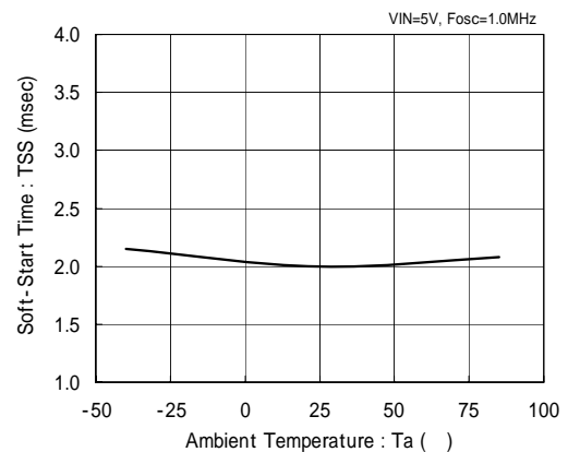
XC9220/21series
