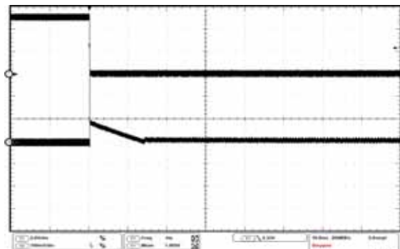
XC9220x095xx ( 500kHz, PWM制御 ) VIN=10.0V, VOUT=3.3V VOUT : 100mV/div, Time : 10msec/div
