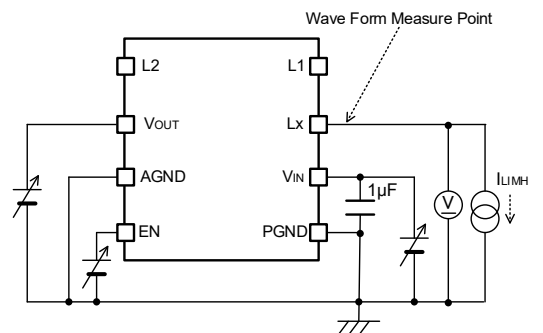
< Circuit No.⑥ >
