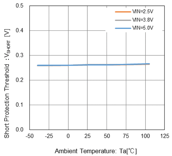
(19) Short Protection Voltage vs. Ambient Temperature
